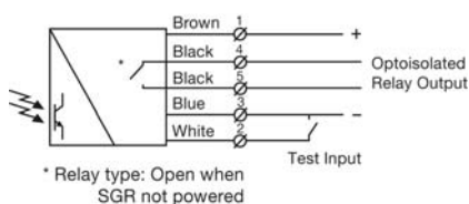
Receiver SGR 15 with solid state relay output.
